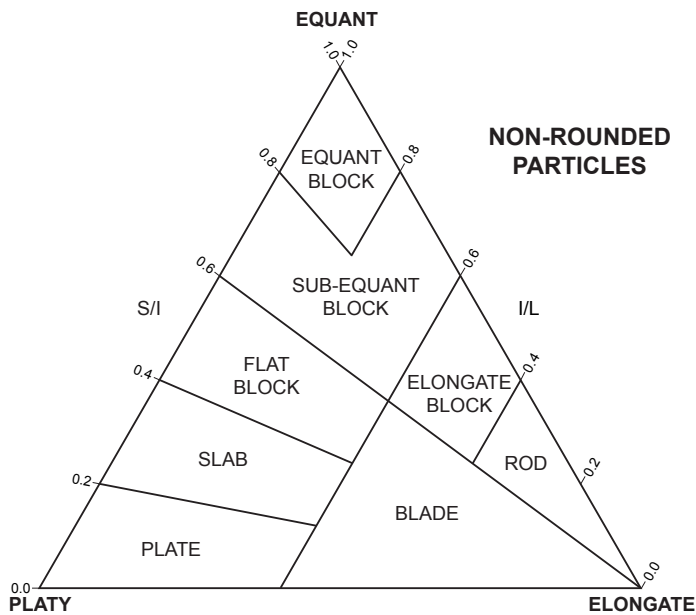
Sneed and Folk (1958) diagrams
