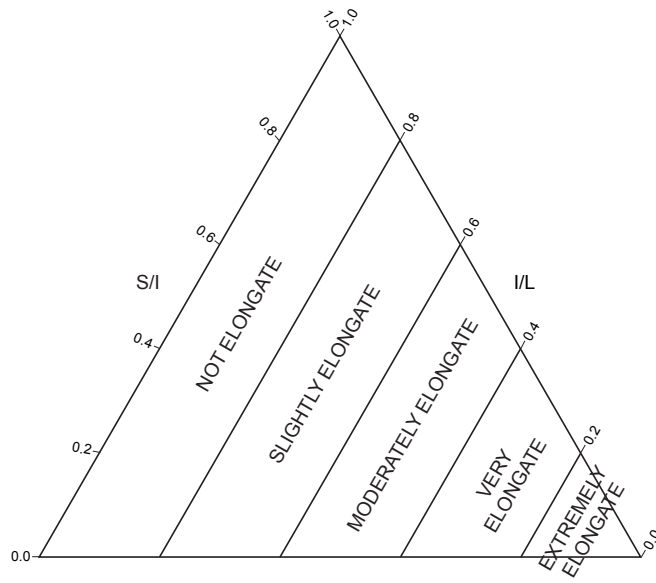
Sneed and Folk (1958) diagrams
